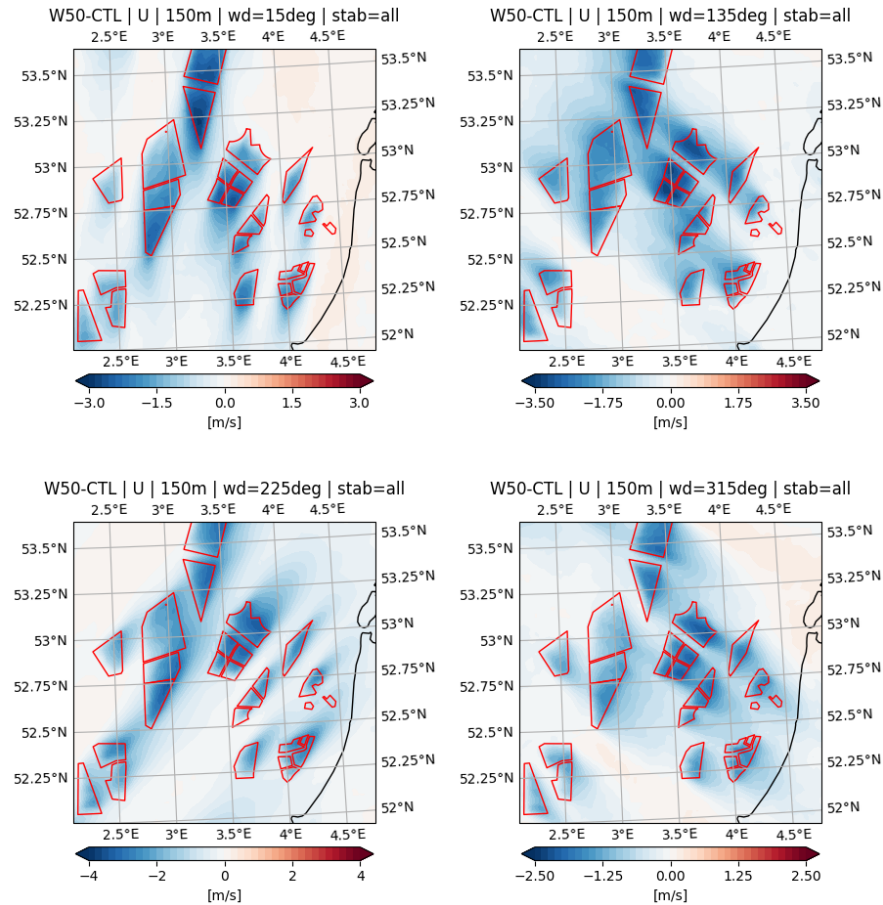
Figure 14. Velocity deficits (W50-CTL, 150-m wind speed) as modeled by HARMONIE-AROME for the year 2020 for four 30-degree wind direction sectors.
